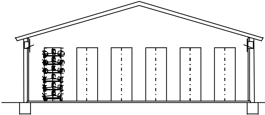
Figure 3-3: Jet ventilation: one row of air inlets per side
