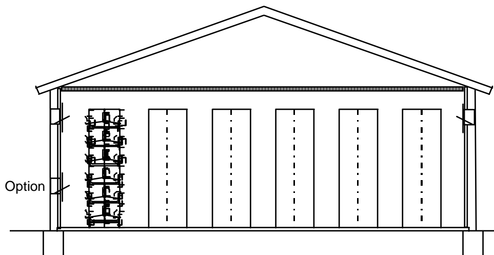
Figure 3-4: diffuse ventilation: one row of air inlets per side
